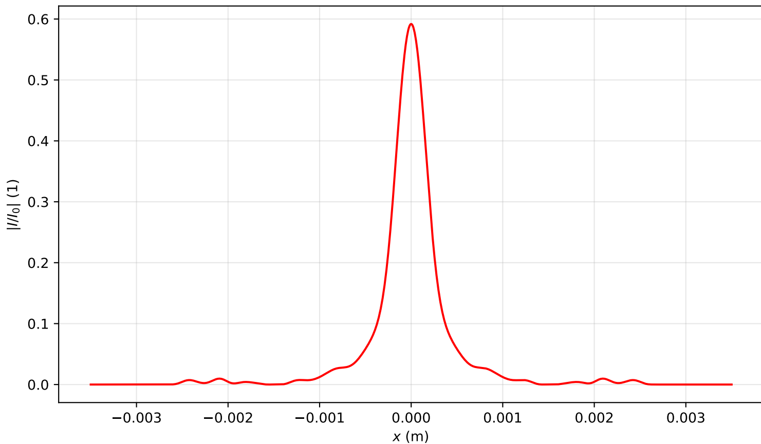
Intensity profile I(x, y = 0, z = 2.707)/I_0 , P_{in}=4.0P_{cr} , artificial time
